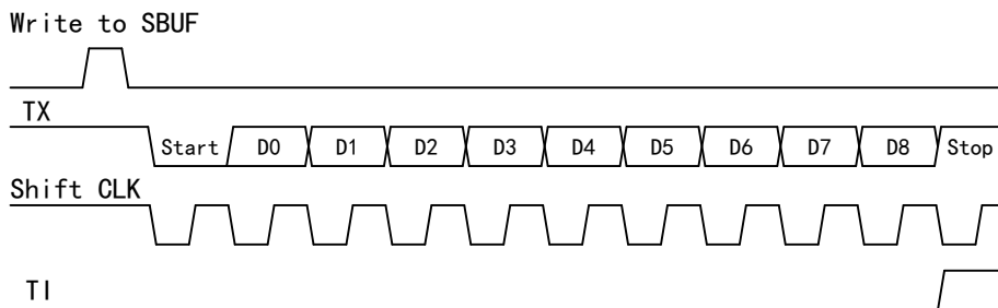
Send Timing of Mode 2
